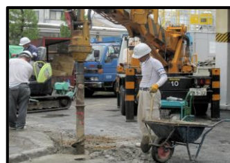
ICCP Anode Installation
