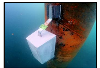
Aluminum Anode on Piles
