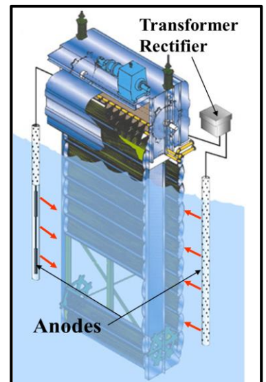
ICCP System
